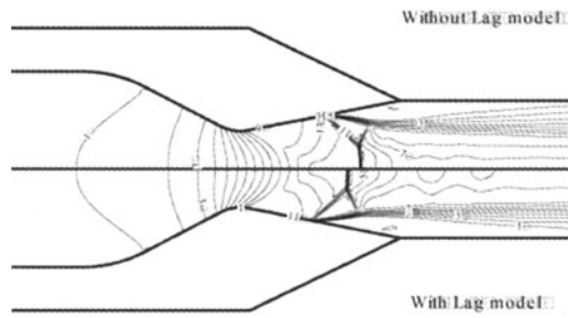
Fig. 4. Mach contour with lag and without lag model ( NPR=2.4 ). Mach contour range is from 0.24-1.71, dMa=0.24 .
