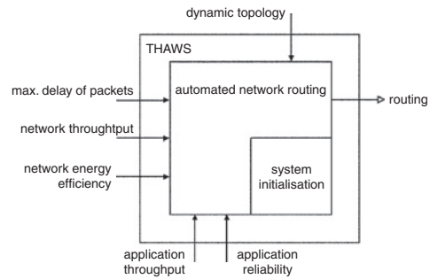
Fig. 2 Automated network routing components and interfaces schematic
